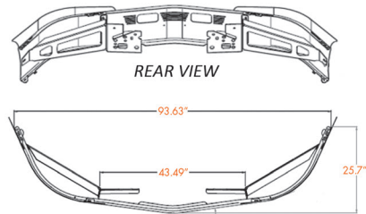
EY-0011-16X Tow pins, open vent
