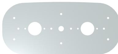
VP170106 DUAL WATERMELON INTERIOR PLATE W/SWITCH HOLE (389 DOME LIGHT)
